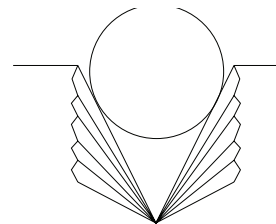
Knurled (R) Groove for flux core wires
