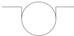
U Groove for soft wires (Aluminium)
